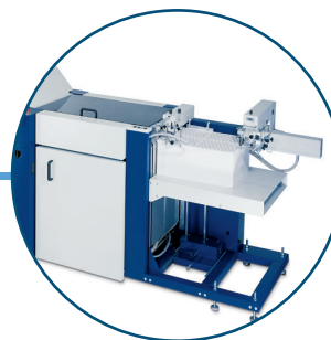
FD 2350 Pile Loader High-capacity elevating deck holds up to 3,500 forms
